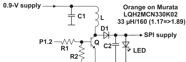
Figure 8. Booster Converter Type A
