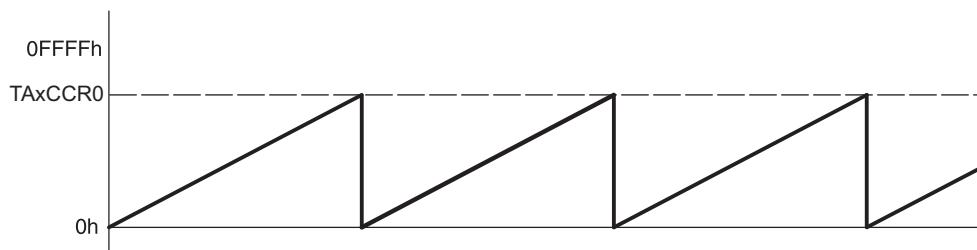
Figure 6-2. Up Mode
